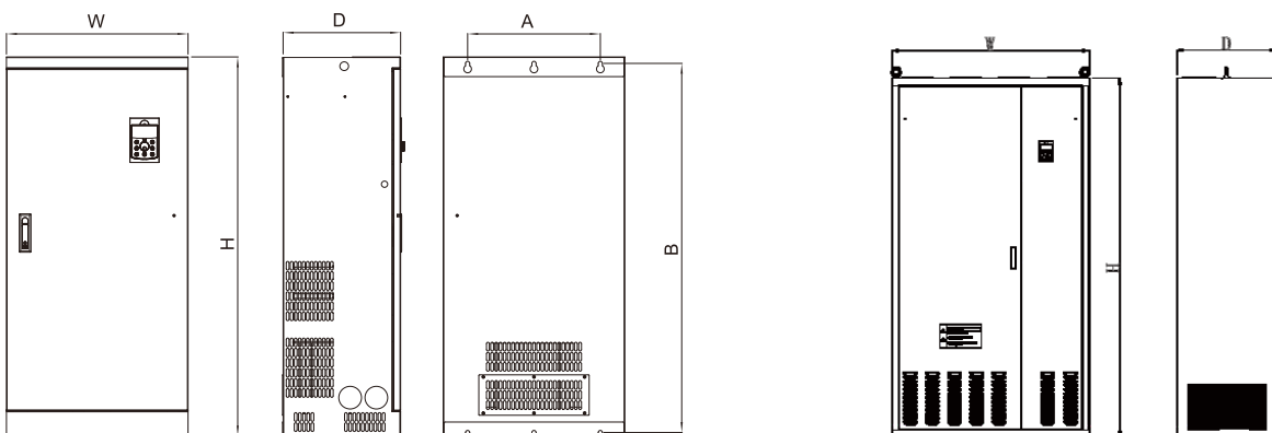
380V(4T) 160~400kW Inverter Dimensions and Installation Dimensions Schematic
