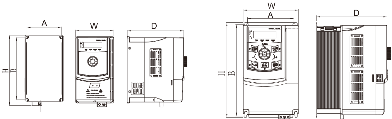
220V (3S) 2.2kW and Below Plastic Enclosure Dimensions and Installation Dimensions Schematic 380V (4T) 15kW and Below Plastic Enclosure Dimensions and Installation Dimensions Schematic
