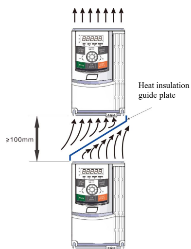
Figure 3-2. Installation diagram of VFD
