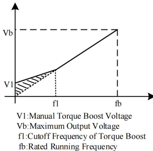
Figure 5-4. Manual Torque Lifting Diagram
