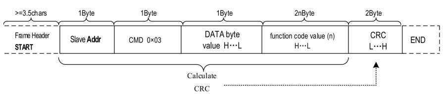
Host write command frame
