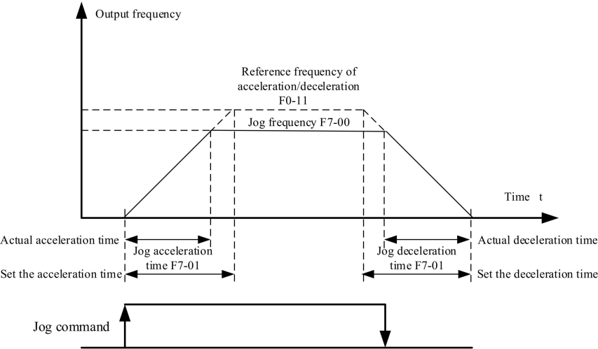
Figure 4-14. Inching Operation Diagram
