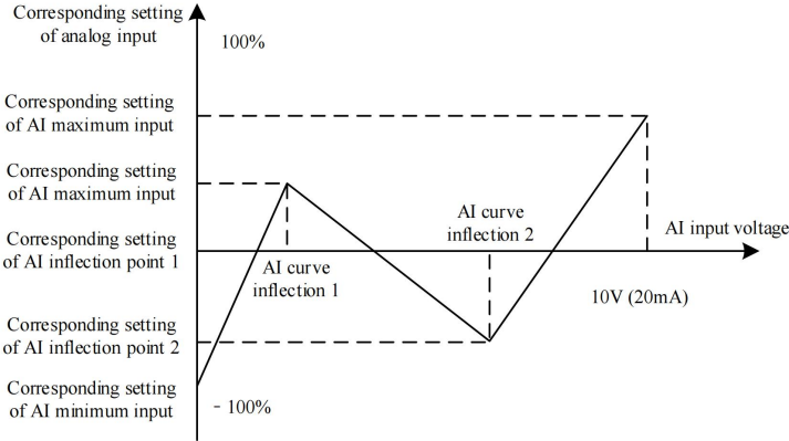
Figure 5-30 Schematic Diagram of Multi-point Curve
