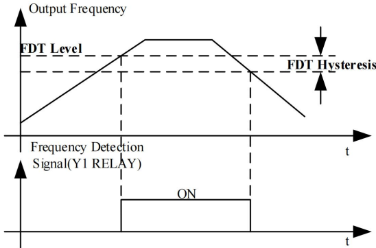
Figure 5-15. FDT Level Diagram
