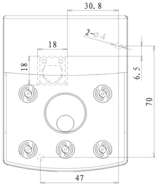
Figure 2-11. Installation Dimension Diagram of External Keyboard Without Tray
