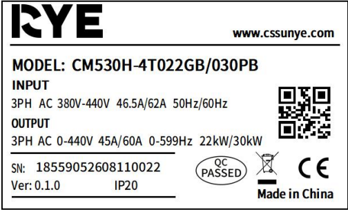
Figure 2-2. Nameplate
