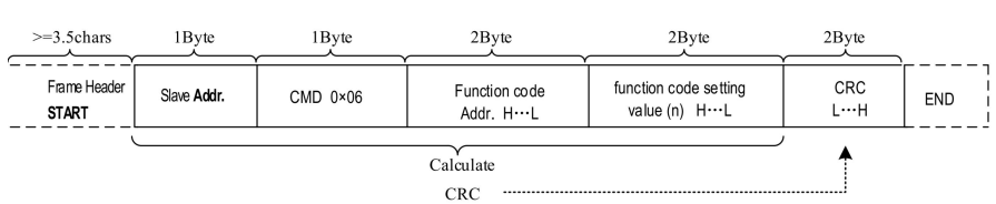
Slave machine write response frame
