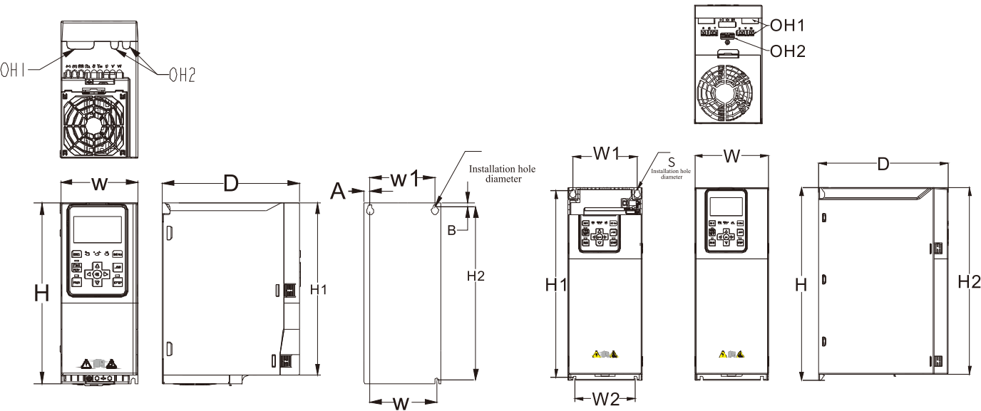
(C2 ~ C3) 380V(4T) Schematic diagram of the plastics shell installation dimensions under 15kW
