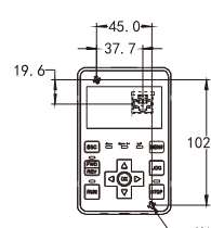
Installation dimension diagram of external keyboard without tray
