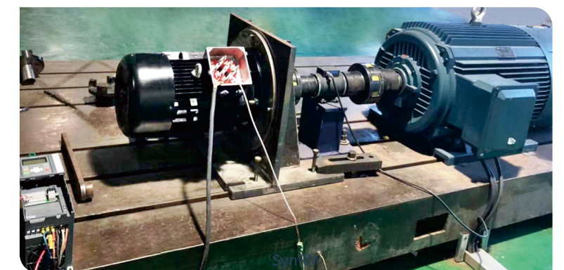
The synchronous reluctance motor control is implemented to allow the VFDs to be applicable for various reluctance motors
