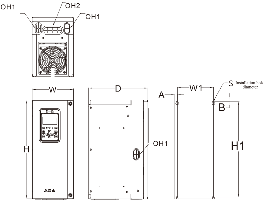
(C5) 380V(4T) Schematic Diagram of the Sheet Metal Chassis Installation Dimensions of 37 to 45 kW
