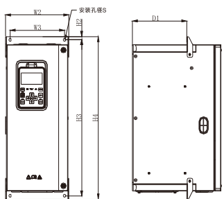
( C5 ) The dimensions of the wall-penetrating installation holes for CM680 VFDs 37 ~ 45kW
