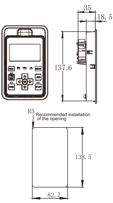
Installation dimension diagram of external keyboard with tray
