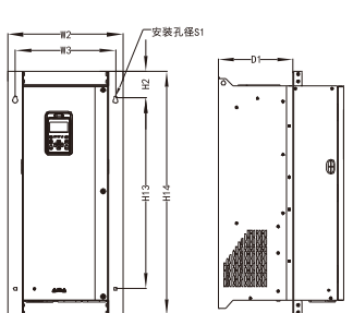
( C6—C8 ) The dimensions of the wall-penetrating installation holes for CM680 VFDs 55 ~ 185kW
